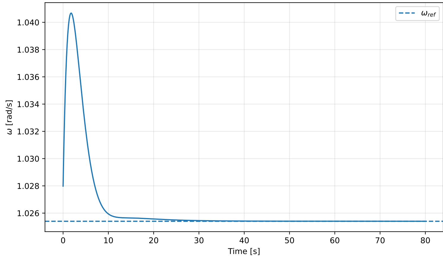
Above-rated rotor-speed response at V_0 = 16.0 m/s
